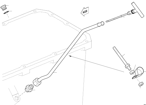
OIL FILLER NECK UPC.06G04 1375
